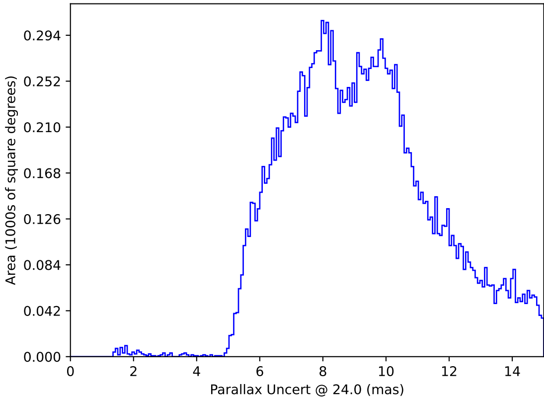
too_elab_heavy_r32_d2_ugrizy_v3.4_10yrs : Parallax Uncert @ 24.0
