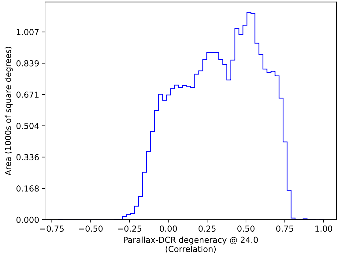
too_elab_heavy_r32_d2_ugrizy_v3.4_10yrs : Parallax-DCR degeneracy @ 24.0
