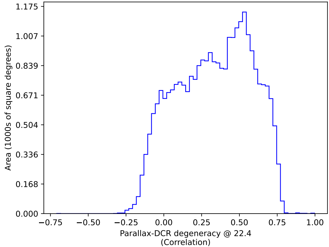
too_elab_heavy_r32_d2_ugrizy_v3.4_10yrs : Parallax-DCR degeneracy @ 22.4
