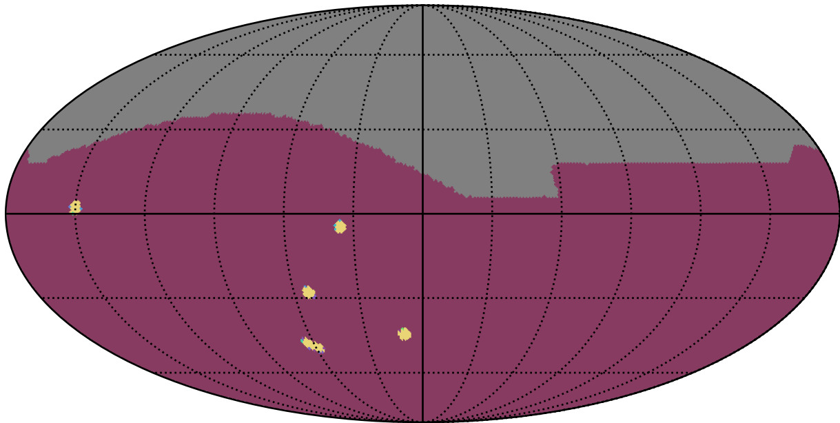
too_elab_heavy_r32_d2_ugrizy_v3.4_10yrs : NumberOfQuickRevisits
