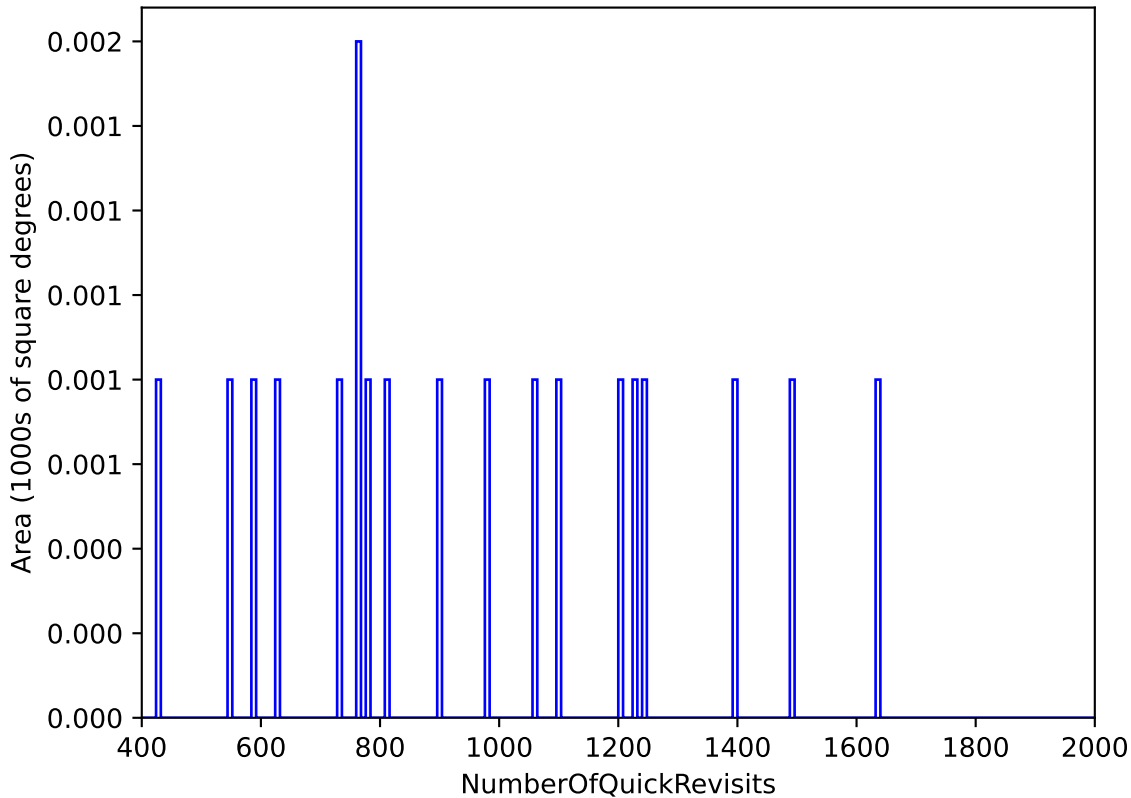
too_elab_heavy_r32_d2_ugrizy_v3.4_10yrs : NumberOfQuickRevisits
