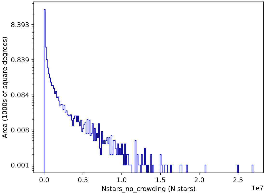
too_elab_heavy_r32_d2_ugrizy_v3.4_10yrs i: Nstars_no_crowding
