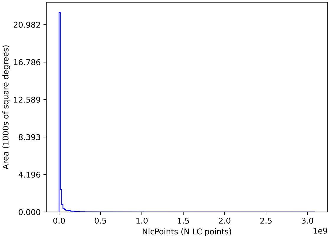
too_elab_heavy_r32_d2_ugrizy_v3.4_10yrs : NlcPoints
