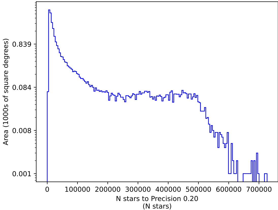
too_elab_heavy_r32_d2_ugrizy_v3.4_10yrs r: N stars to Precision 0.20
