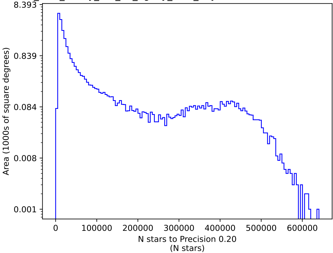
too_elab_heavy_r32_d2_ugrizy_v3.4_10yrs i: N stars to Precision 0.20
