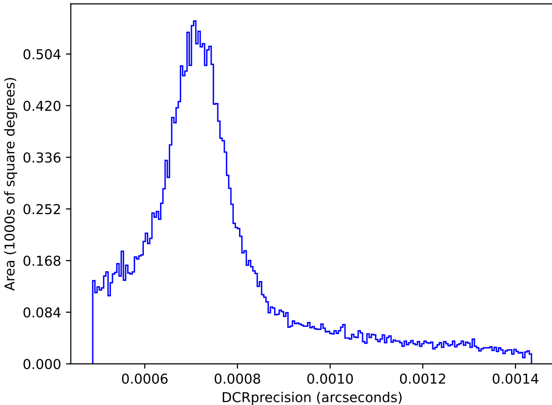
too_elab_heavy_r32_d2_ugrizy_v3.4_10yrs : DCRprecision
