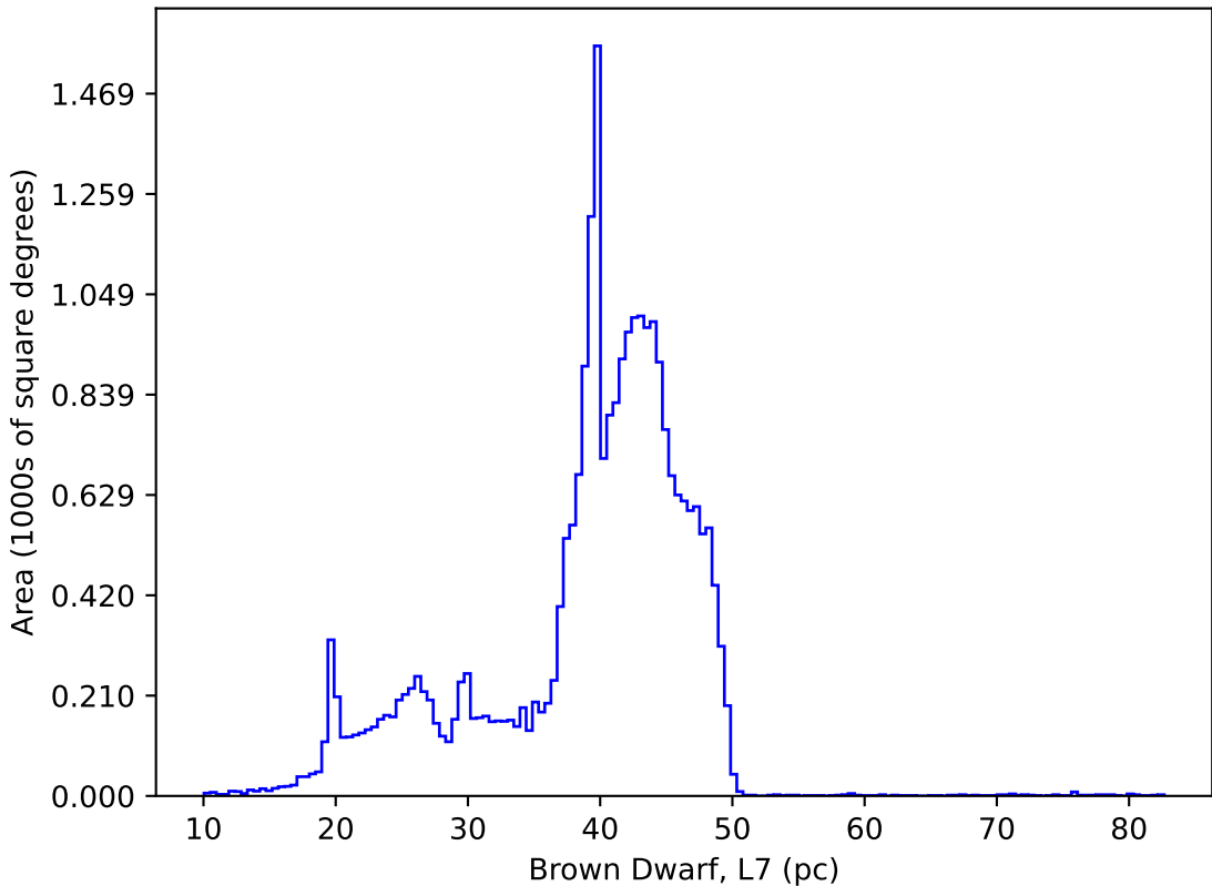
too_elab_heavy_r32_d2_ugrizy_v3.4_10yrs : Brown Dwarf, L7
