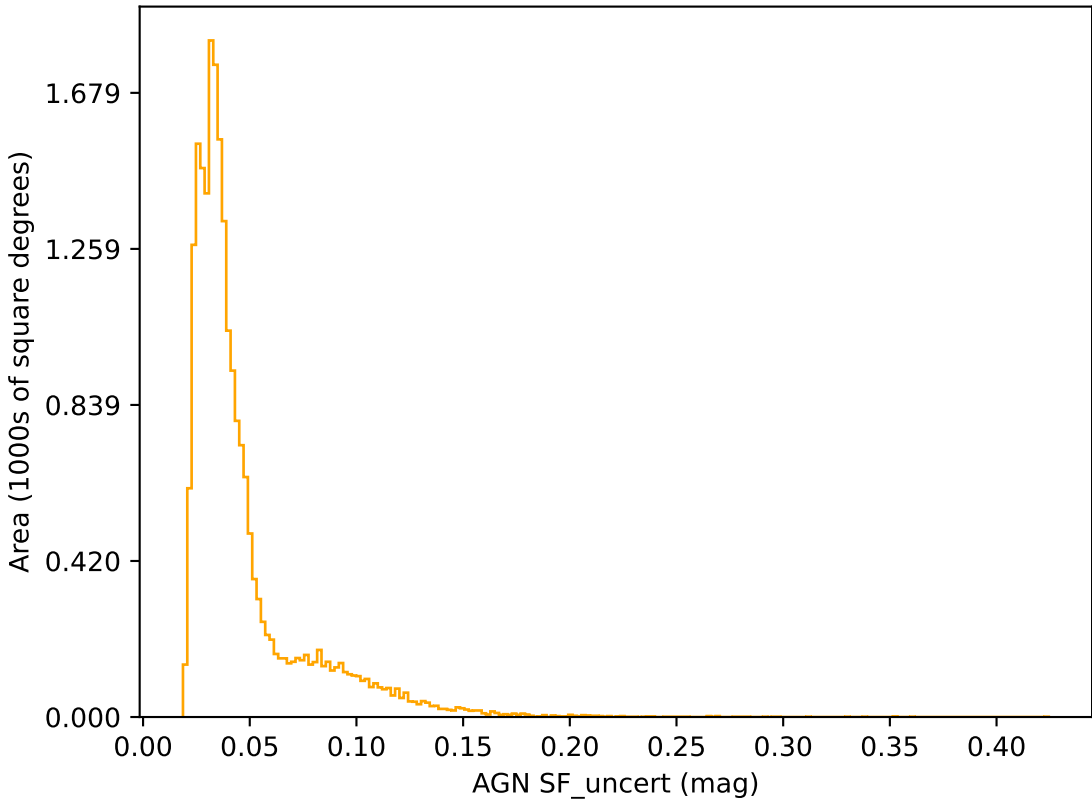
too_elab_heavy_r32_d2_ugrizy_v3.4_10yrs r band: AGN SF_uncert
