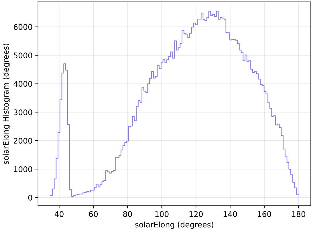
too_elab_heavy_r32_d2_ugrizy_v3.4_10yrs WFD z band: solarElong Histogram
