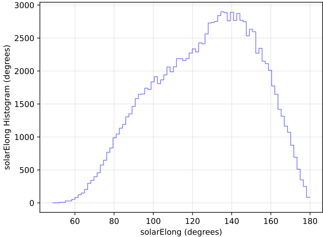
too_elab_heavy_r32_d2_ugrizy_v3.4_10yrs WFD u band: solarElong Histogram
