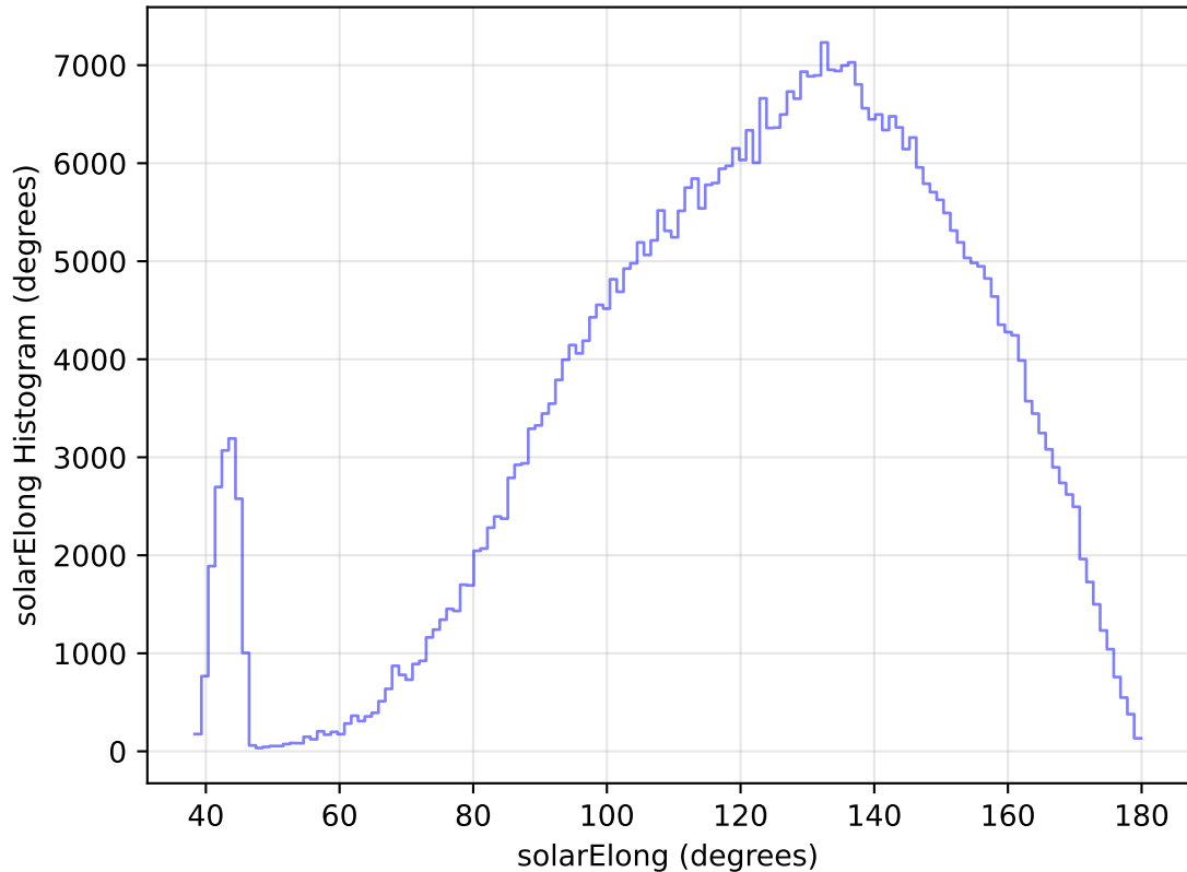
too_elab_heavy_r32_d2_ugrizy_v3.4_10yrs WFD r band: solarElong Histogram
