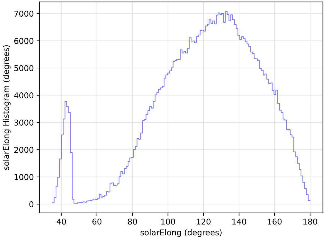
too_elab_heavy_r32_d2_ugrizy_v3.4_10yrs WFD i band: solarElong Histogram
