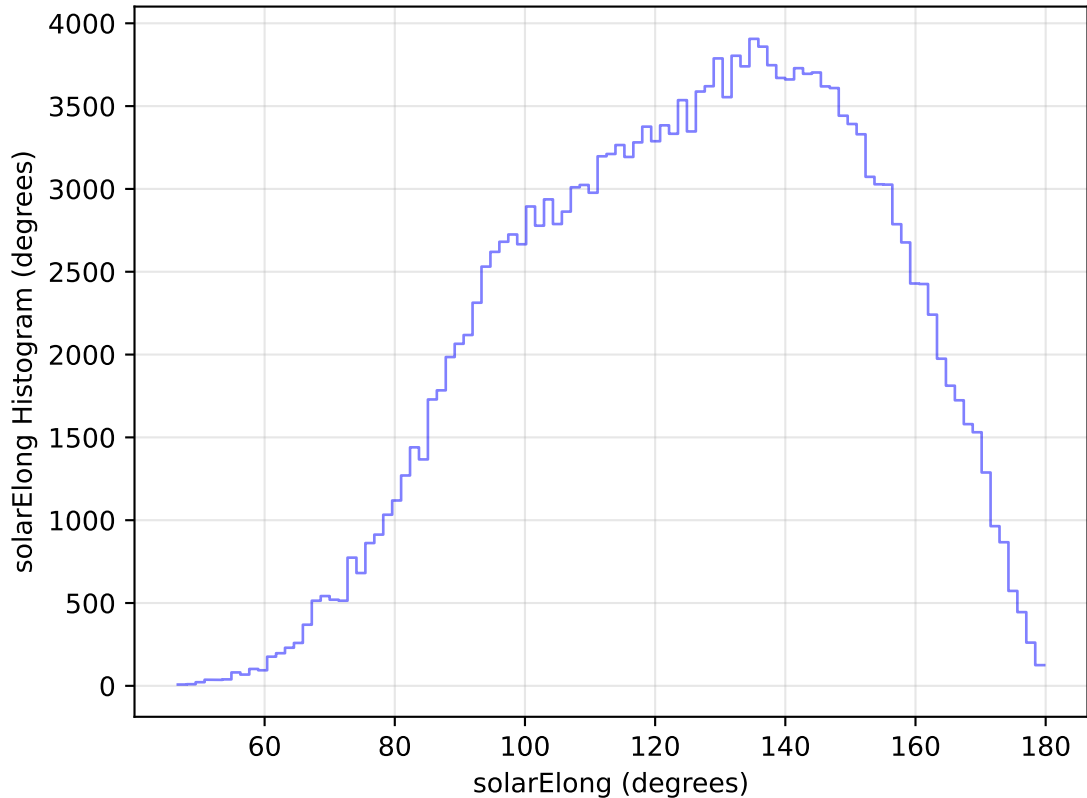
too_elab_heavy_r32_d2_ugrizy_v3.4_10yrs WFD g band: solarElong Histogram
