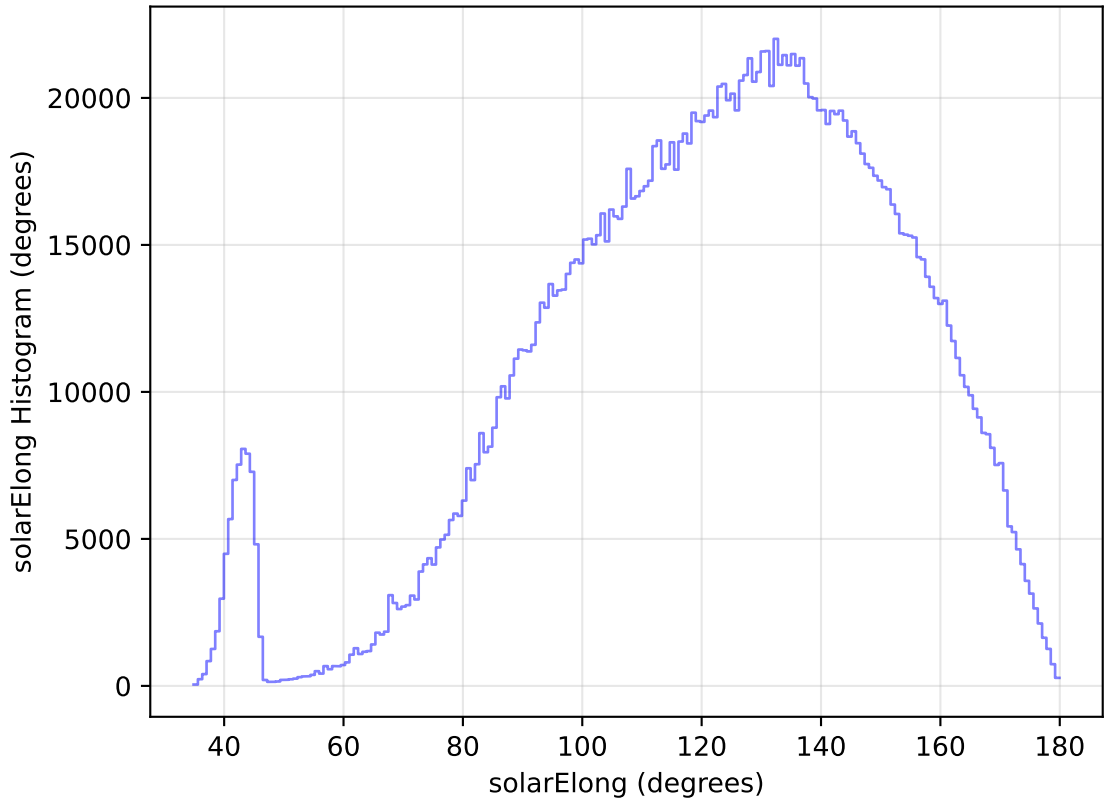
too_elab_heavy_r32_d2_ugrizy_v3.4_10yrs WFD all bands: solarElong Histogram
