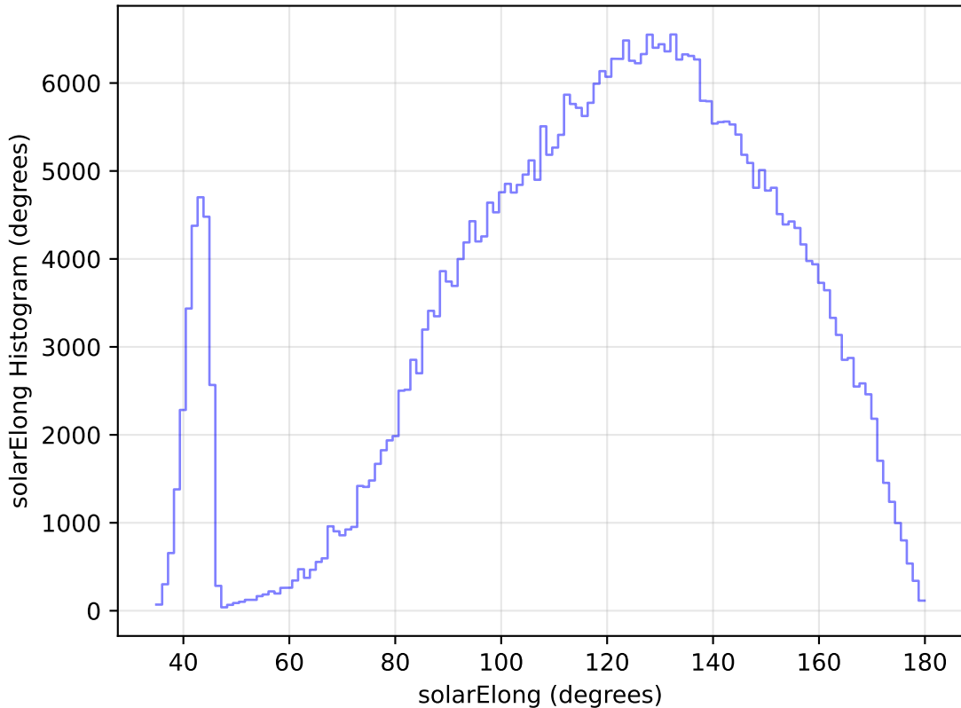
too_elab_heavy_r32_d2_ugrizy_v3.4_10yrs All sky z band: solarElong Histogram
