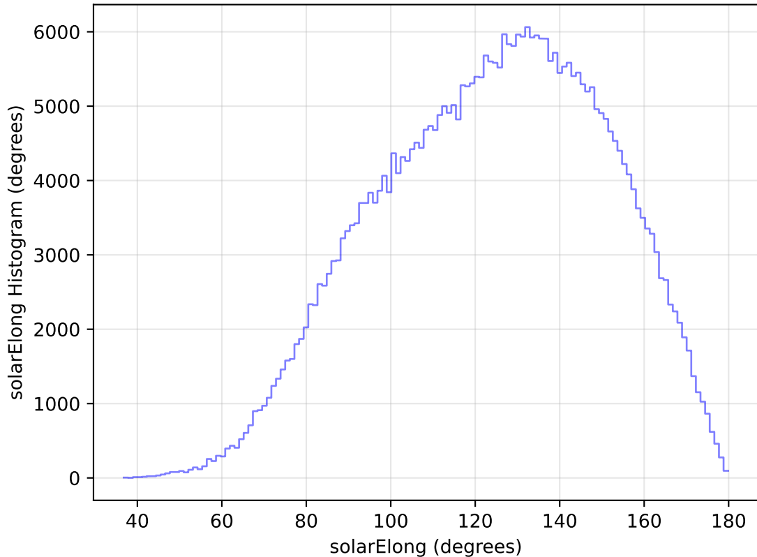
too_elab_heavy_r32_d2_ugrizy_v3.4_10yrs All sky y band: solarElong Histogram
