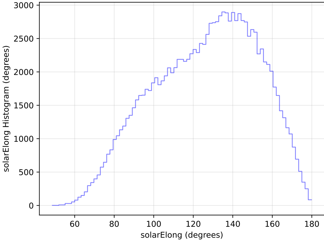
too_elab_heavy_r32_d2_ugrizy_v3.4_10yrs All sky u band: solarElong Histogram
