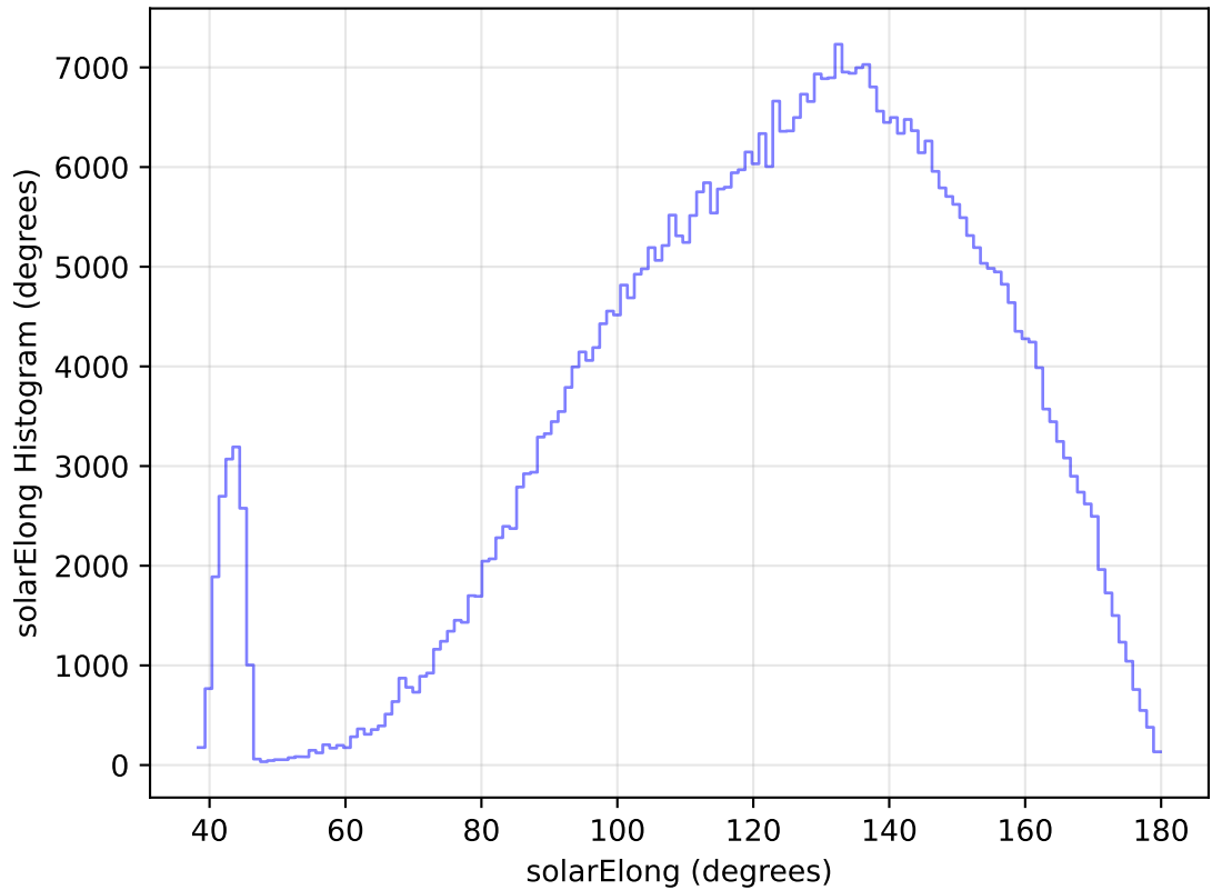
too_elab_heavy_r32_d2_ugrizy_v3.4_10yrs All sky r band: solarElong Histogram
