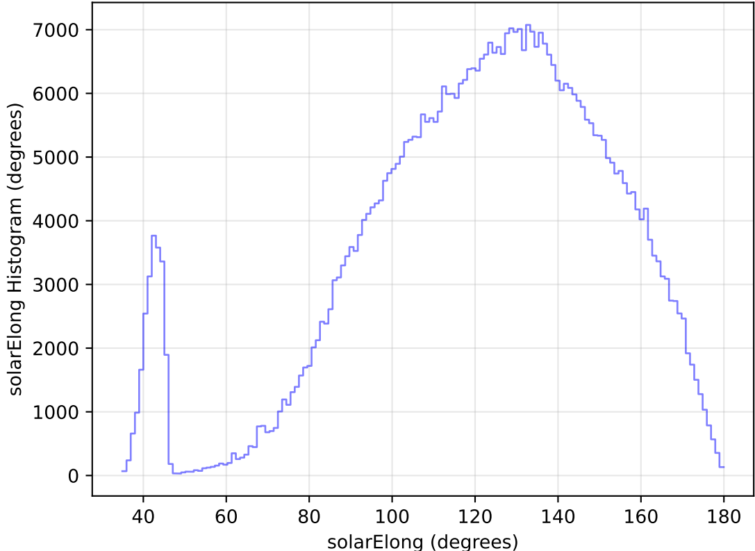
too_elab_heavy_r32_d2_ugrizy_v3.4_10yrs All sky i band: solarElong Histogram
