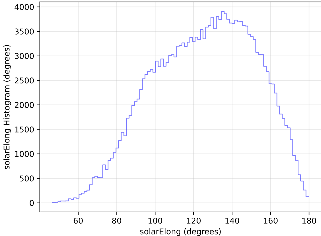
too_elab_heavy_r32_d2_ugrizy_v3.4_10yrs All sky g band: solarElong Histogram
