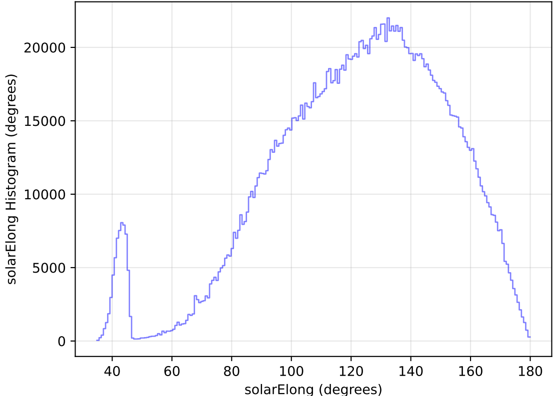
too_elab_heavy_r32_d2_ugrizy_v3.4_10yrs All sky all bands: solarElong Histogram
