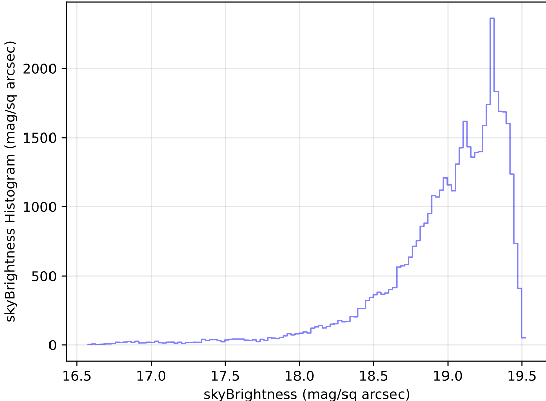
too_elab_heavy_r32_d2_ugrizy_v3.4_10yrs Yr 1 z band: skyBrightness Histogram
