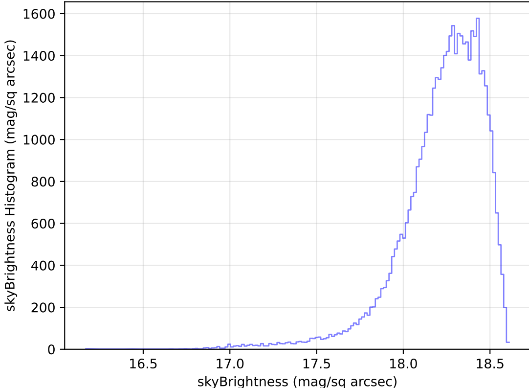
too_elab_heavy_r32_d2_ugrizy_v3.4_10yrs Yr 1 y band: skyBrightness Histogram
