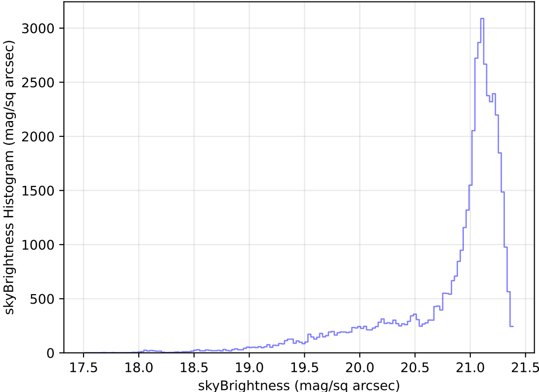
too_elab_heavy_r32_d2_ugrizy_v3.4_10yrs Yr 1 r band: skyBrightness Histogram
