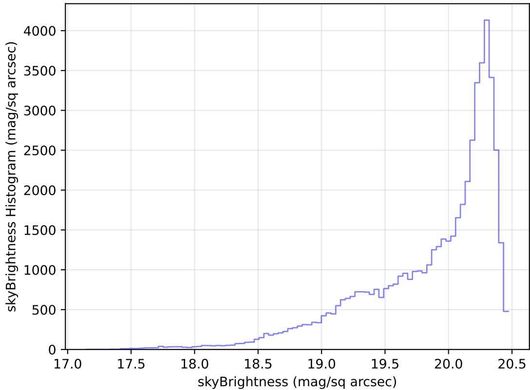
too_elab_heavy_r32_d2_ugrizy_v3.4_10yrs Yr 1 i band: skyBrightness Histogram
