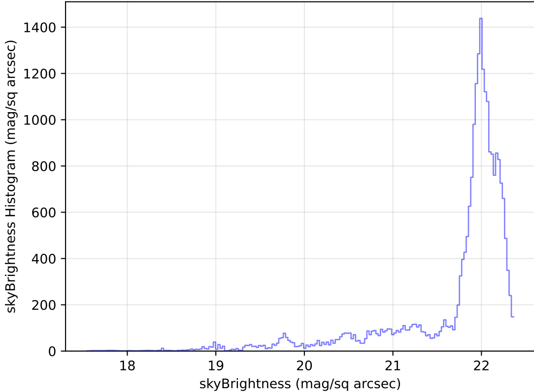
too_elab_heavy_r32_d2_ugrizy_v3.4_10yrs Yr 1 g band: skyBrightness Histogram
