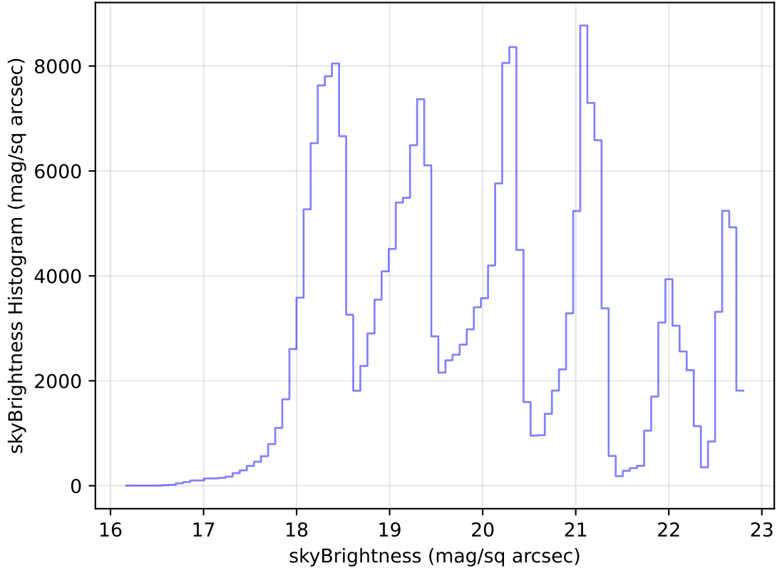
too_elab_heavy_r32_d2_ugrizy_v3.4_10yrs Yr 1 all bands: skyBrightness Histogram
