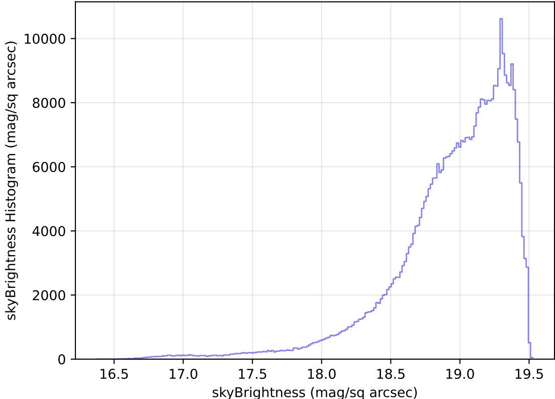
too_elab_heavy_r32_d2_ugrizy_v3.4_10yrs WFD z band: skyBrightness Histogram
