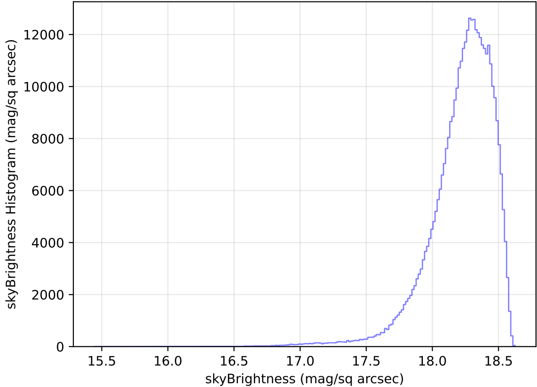
too_elab_heavy_r32_d2_ugrizy_v3.4_10yrs WFD y band: skyBrightness Histogram
