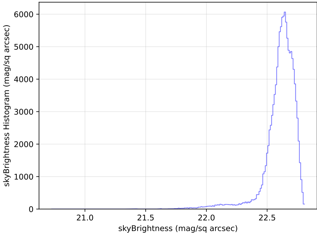
too_elab_heavy_r32_d2_ugrizy_v3.4_10yrs WFD u band: skyBrightness Histogram
