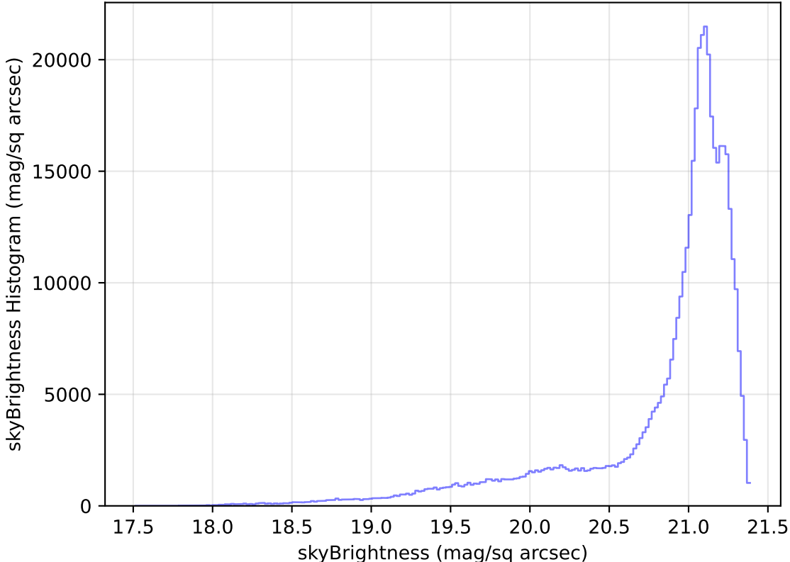
too_elab_heavy_r32_d2_ugrizy_v3.4_10yrs WFD r band: skyBrightness Histogram
