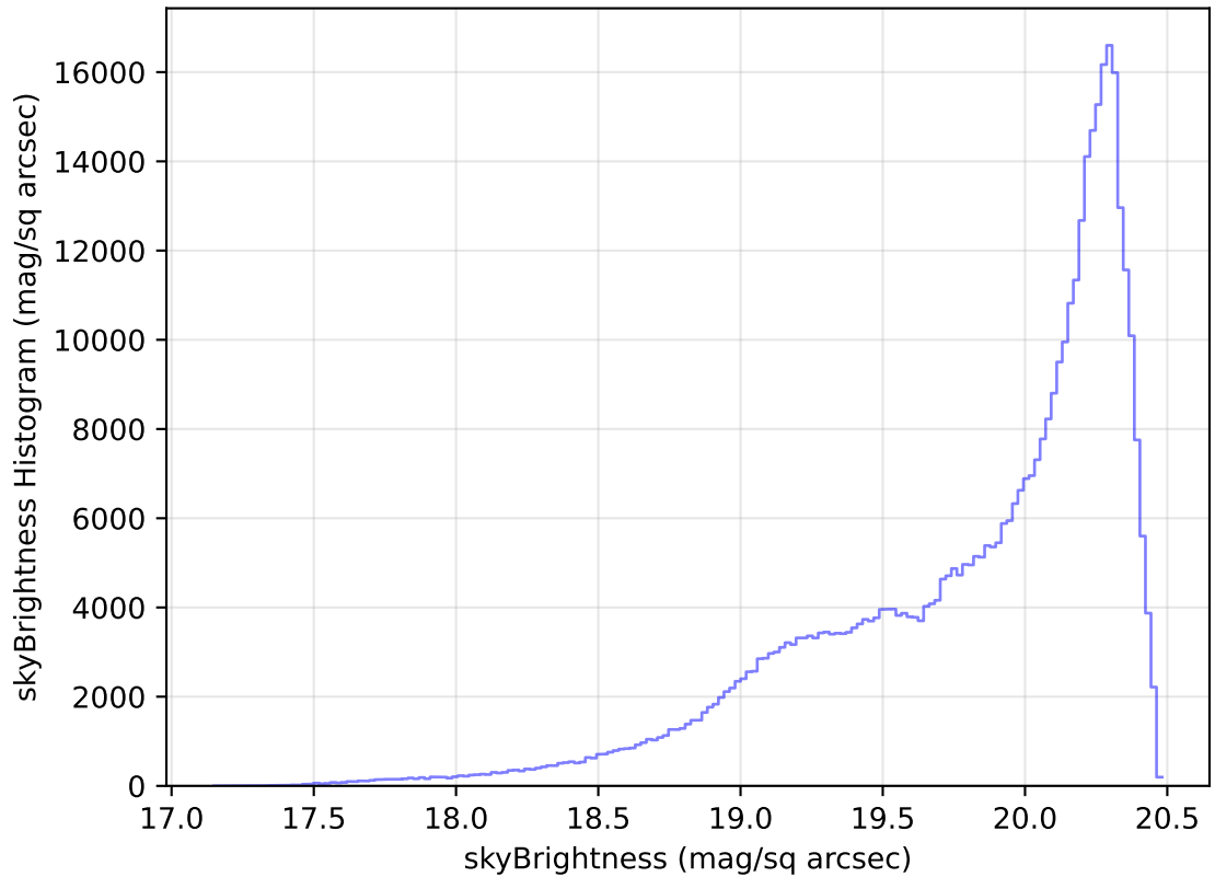
too_elab_heavy_r32_d2_ugrizy_v3.4_10yrs WFD i band: skyBrightness Histogram
