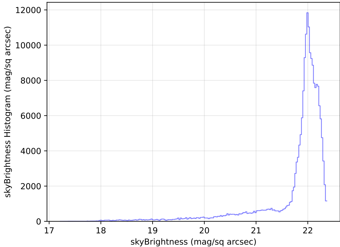
too_elab_heavy_r32_d2_ugrizy_v3.4_10yrs WFD g band: skyBrightness Histogram
