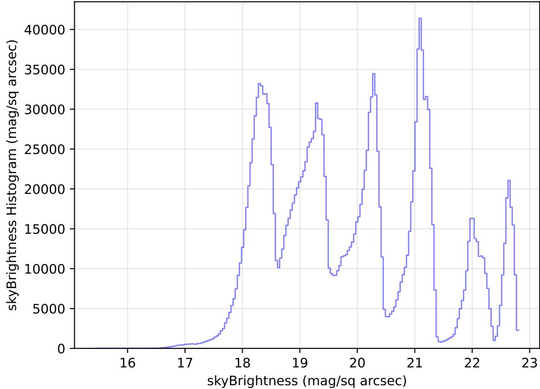
too_elab_heavy_r32_d2_ugrizy_v3.4_10yrs WFD all bands: skyBrightness Histogram
