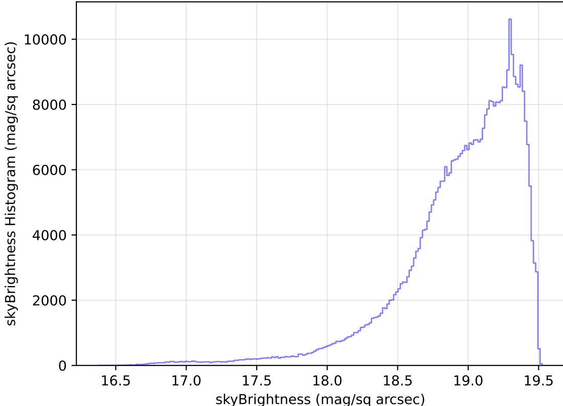
too_elab_heavy_r32_d2_ugrizy_v3.4_10yrs All sky z band: skyBrightness Histogram
