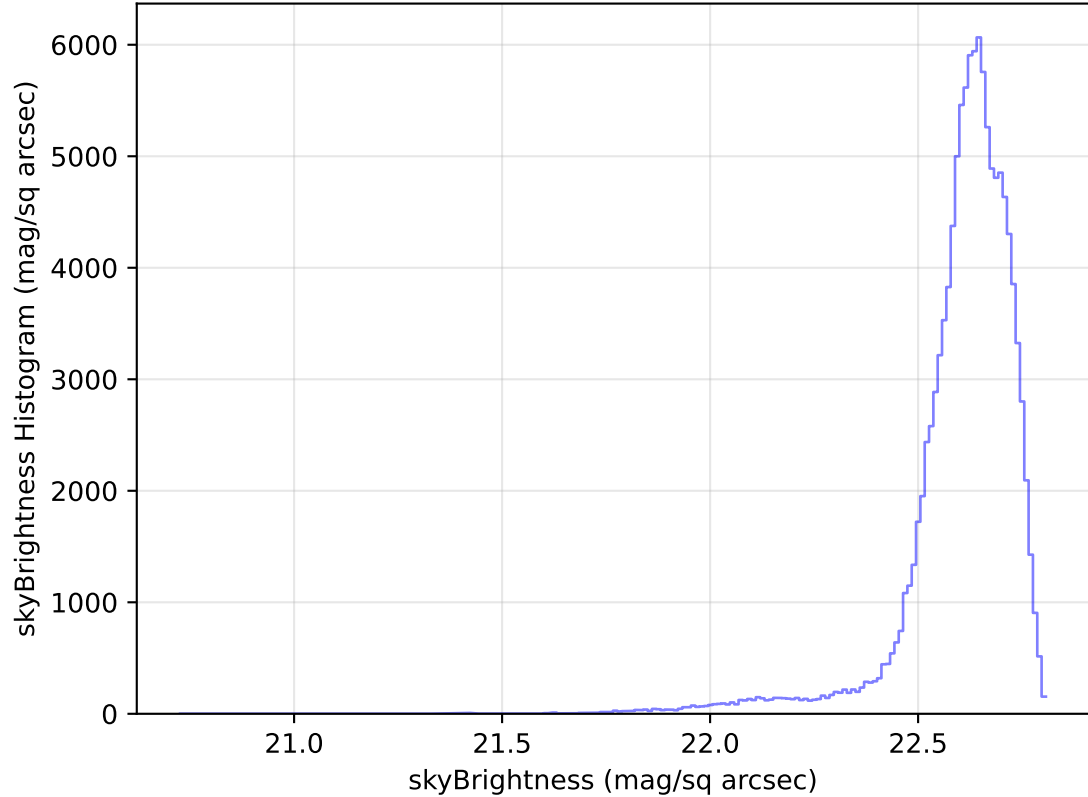
too_elab_heavy_r32_d2_ugrizy_v3.4_10yrs All sky u band: skyBrightness Histogram
