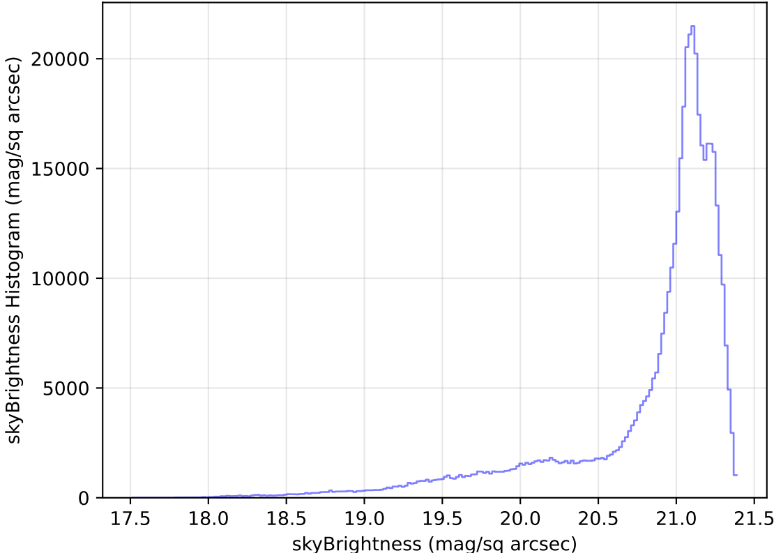
too_elab_heavy_r32_d2_ugrizy_v3.4_10yrs All sky r band: skyBrightness Histogram
