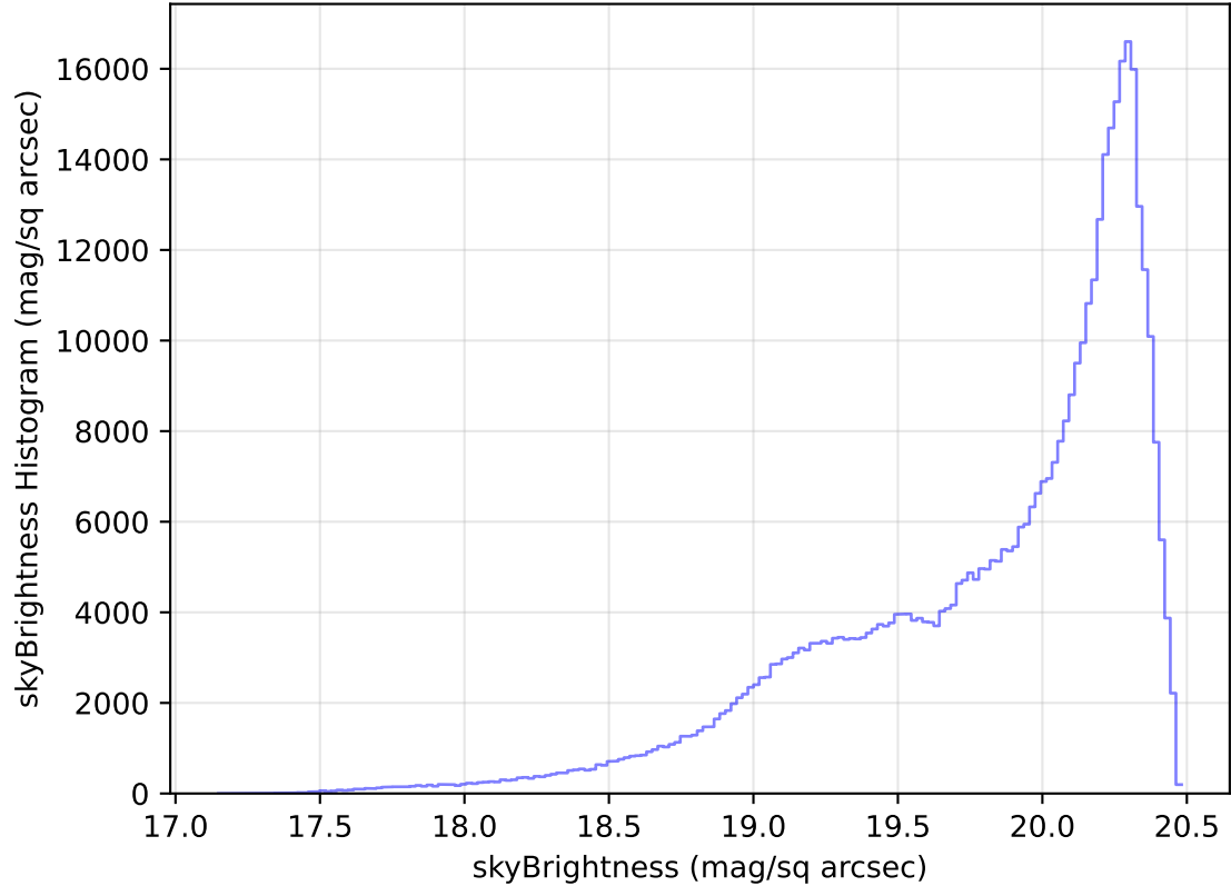
too_elab_heavy_r32_d2_ugrizy_v3.4_10yrs All sky i band: skyBrightness Histogram
