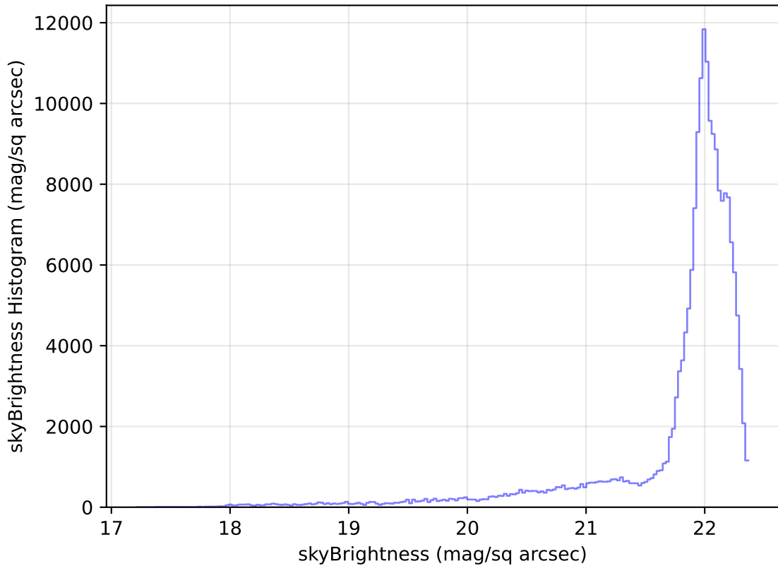
too_elab_heavy_r32_d2_ugrizy_v3.4_10yrs All sky g band: skyBrightness Histogram
