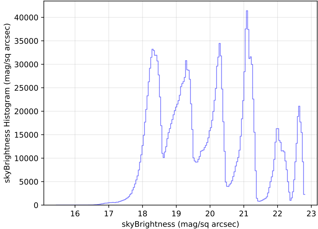
too_elab_heavy_r32_d2_ugrizy_v3.4_10yrs All sky all bands: skyBrightness Histogram
