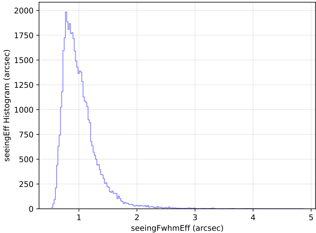
too_elab_heavy_r32_d2_ugrizy_v3.4_10yrs Yr 1 z band: seeingEff Histogram
