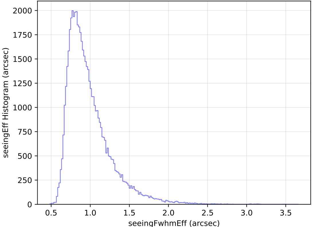
too_elab_heavy_r32_d2_ugrizy_v3.4_10yrs Yr 1 i band: seeingEff Histogram
