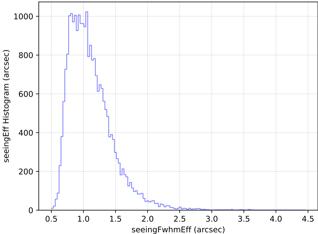
too_elab_heavy_r32_d2_ugrizy_v3.4_10yrs Yr 1 g band: seeingEff Histogram
