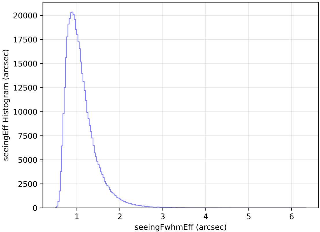
too_elab_heavy_r32_d2_ugrizy_v3.4_10yrs WFD z band: seeingEff Histogram
