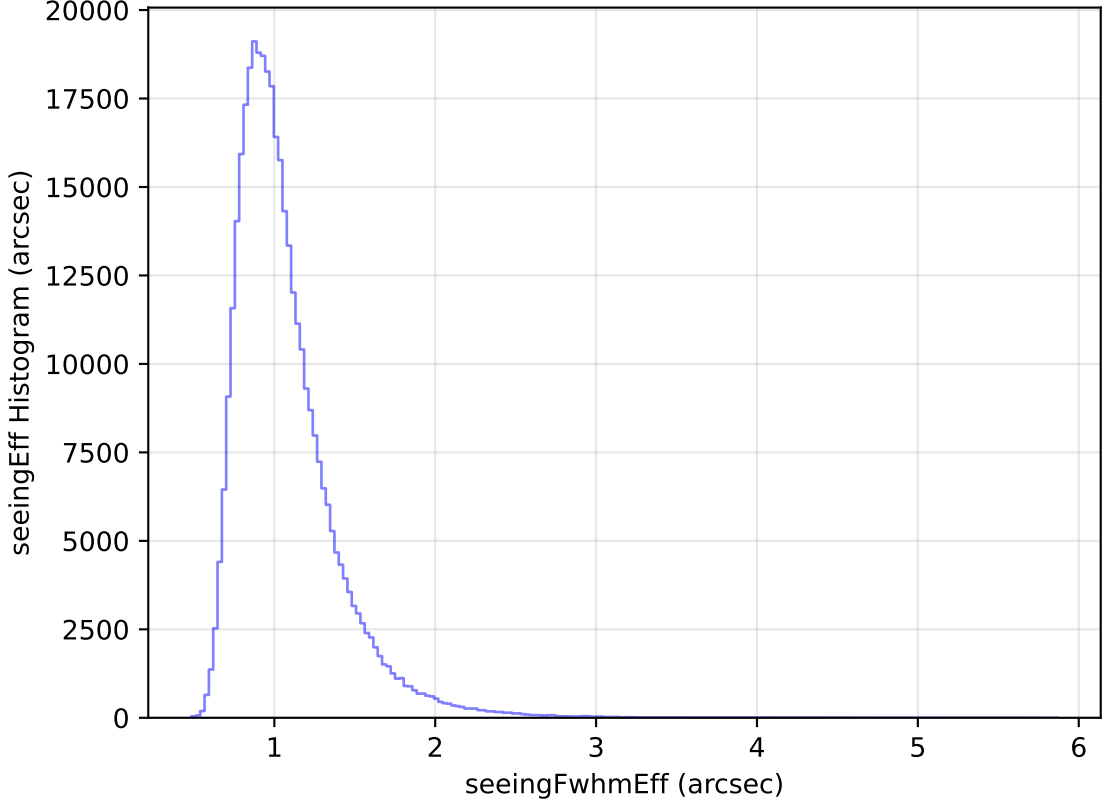
too_elab_heavy_r32_d2_ugrizy_v3.4_10yrs WFD y band: seeingEff Histogram
