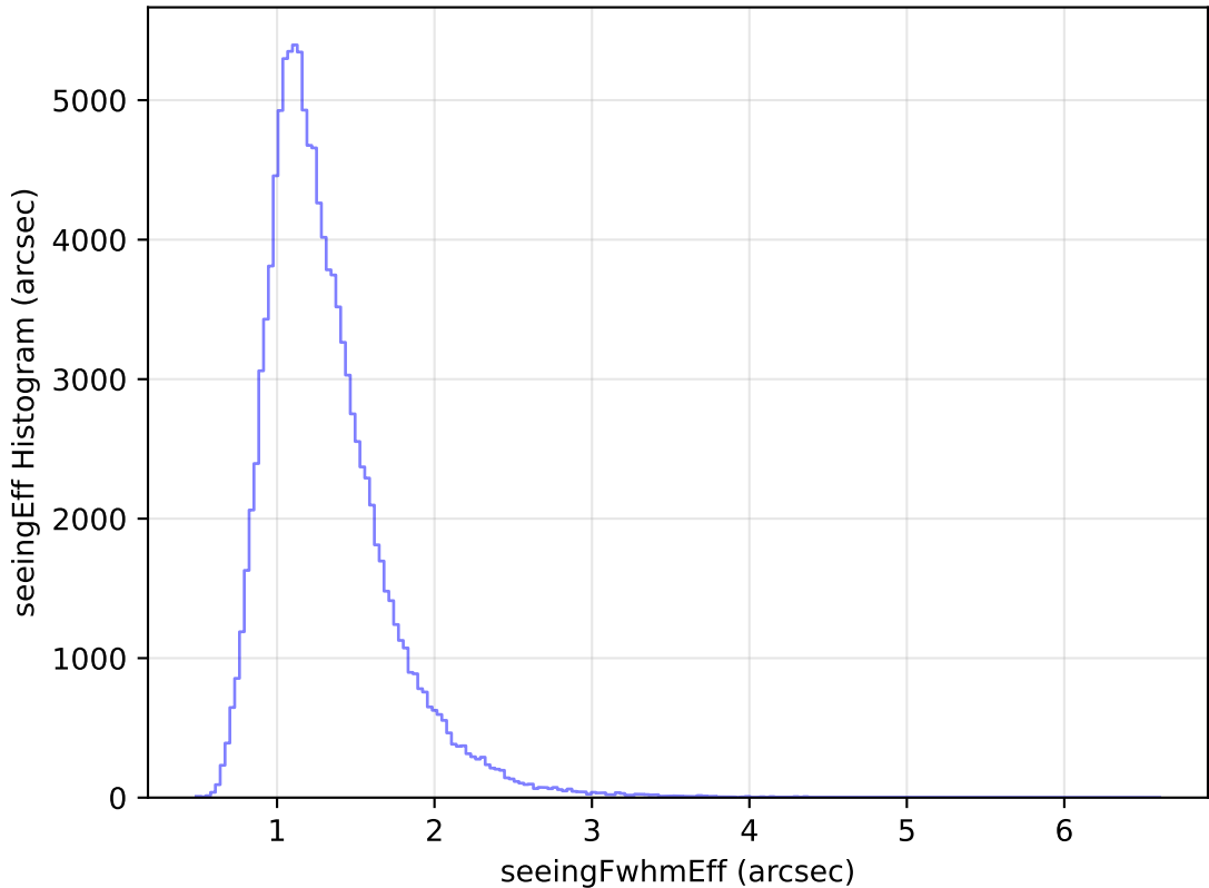
too_elab_heavy_r32_d2_ugrizy_v3.4_10yrs WFD u band: seeingEff Histogram
